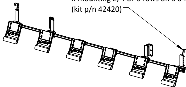
6-Row Layout (6-Row Head)
