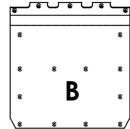
Black - 41768 (22285) End Skid Shoe 17" X 18"
