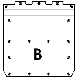
41768 End Skid Shoe 17" X 18" (17) Rivets
